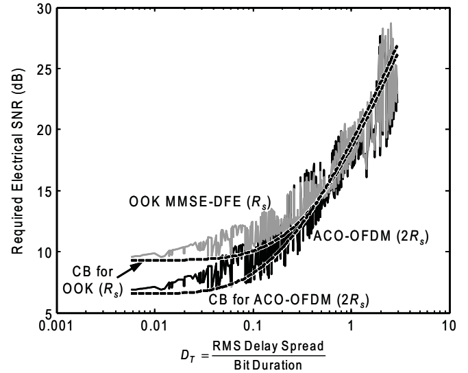
Fig. 8. Electrical SNR required to achieve P_b = 10^{-4} vs. normalized delay spread D_T at bit rates of 50, 100 and 300 Mbit/s (spectral efficiency of 1 bit/symbol) for different modulations formats. The dashed lines correspond to the SNR requirement predicted using the ceiling-bounce (CB) model. The bit allocation granularity is \beta = 0.25 and the symbol rates for ACO-OFDM are twice those for OOK, as indicated.
