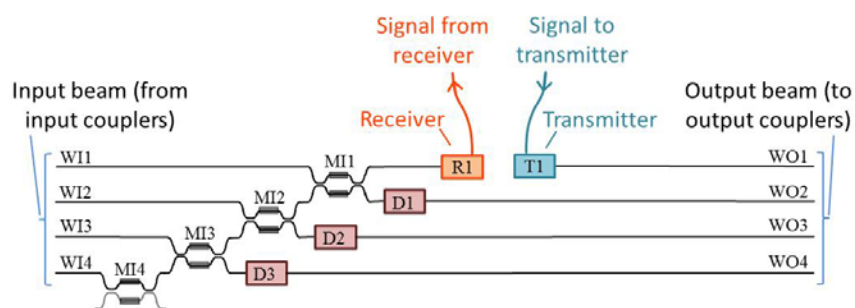
Fig. 4. Simplified device using only a self-aligned mode coupler configuration [26] with added “through” waveguides and mostly-transparent detectors. We could also add dummy MZIs as in the left side of Fig. 2 so all paths have equal numbers of MZIs for loss and path length equality.
