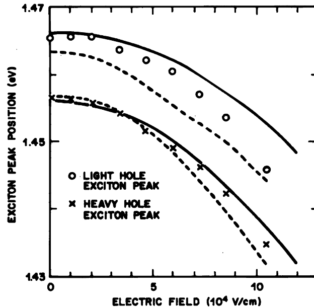
Fig. 11. Measured (points) and calculated (lines) energies of the heavy and light hole exciton peaks in a GaAs/AlGaAs multiple quantum well structure as a function of electric field applied perpendicular to the quantum well layers [9]. The solid and dashed lines are for different values of the band discontinuity offset ratios.
