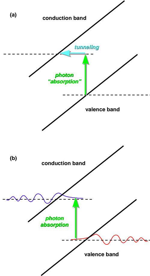
Fig. 4. Illustration of the model pictures of the Franz-Keldysh effect. (a) "photon-assisted tunneling" picture; (b) absorption between eigenstates.
