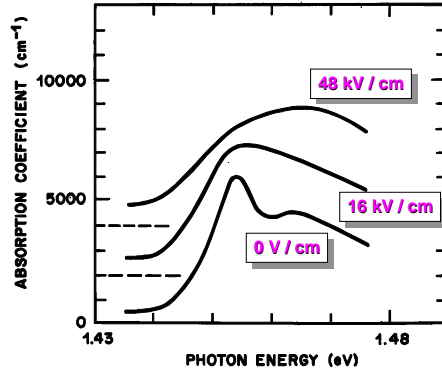
Fig. 8. Absorption of a GaAs/AlGaAs quantum well sample at room temperature for various values of electric field applied in the plane of the quantum well layers (i.e., parallel to the quantum wells). The spectra are shifted vertically for clarity [9].
