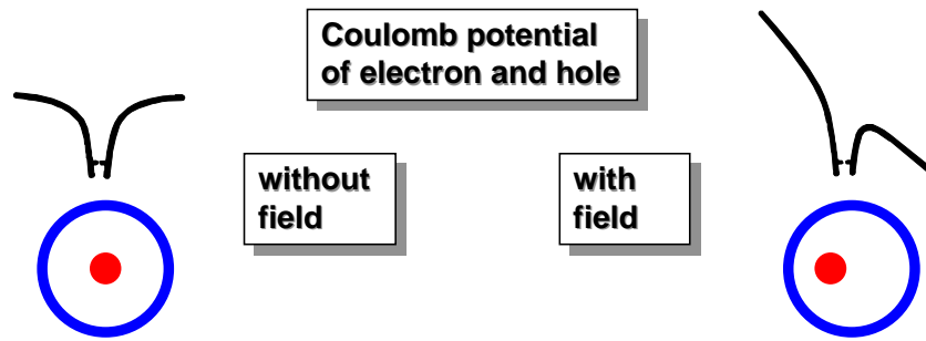
Fig. 7. Illustration of the electron-hole Coulomb potential and the classical orbit of the electron and hole as electric field is applied to the exciton.
