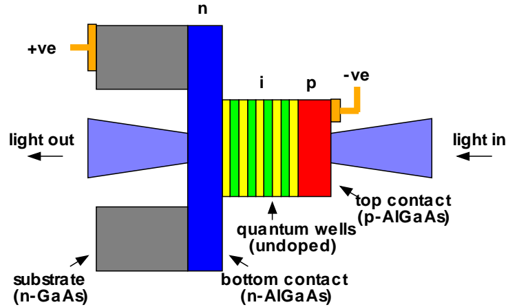
Fig. 10. Structure of a simple quantum well diode. The GaAs/AlGaAs quantum wells are contained in the undoped ( i ) region of a p-i-n diode. The p and n regions are made of AlGaAs, which is transparent at the operating wavelength. Light is shone through the structure, and the diode is reverse biased to apply the electric field perpendicular to the quantum well layers [9].
