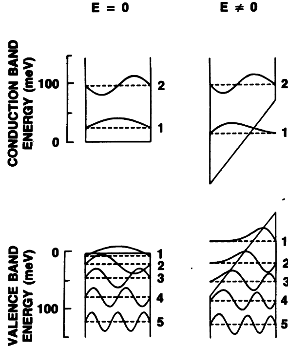
Fig. 6. Energy levels and wavefunctions for valence and conduction states in a quantum well with an electric field applied perpendicular to the layers [8]
