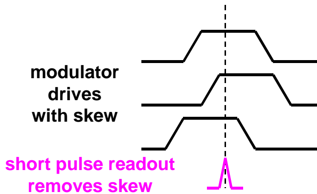
Fig. 2. Illustration of the use of synchronized short pulses to remove skew in the readout of modulators.
