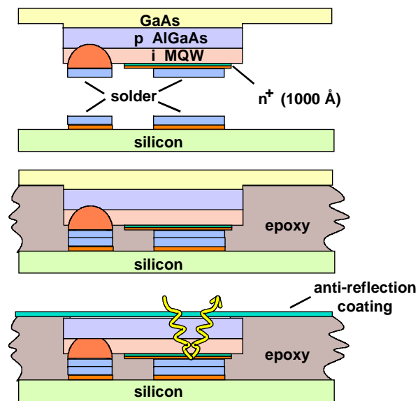
Fig. 12. Illustration of the solder bonding process used for quantum well diodes and silicon integrated circuits.
