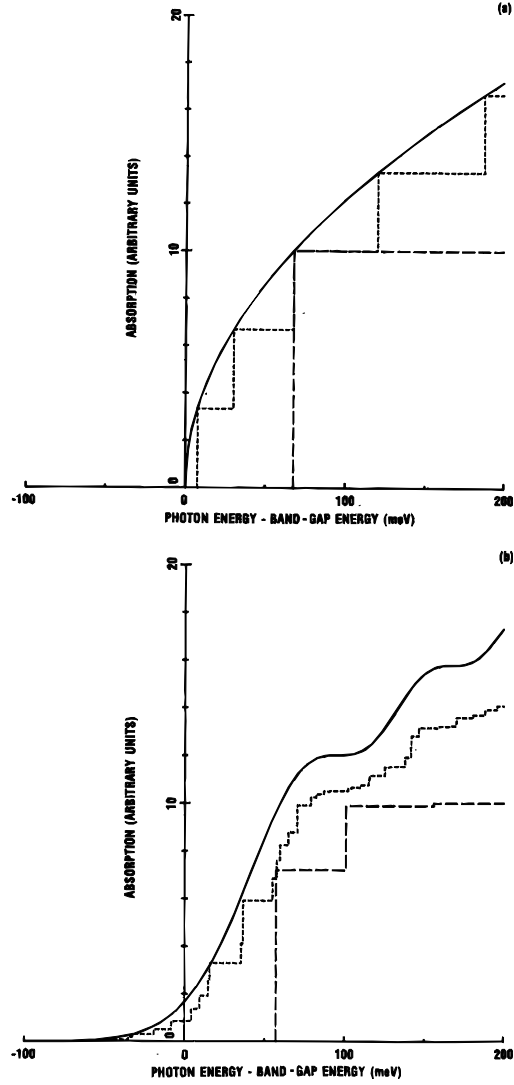
Fig. 5. Form of the theoretical Franz-Keldysh optical absorption (smooth curve) and the quantum well absorption (neglecting excitons) (steps) at 10^5 V/cm [8]. The quantum well calculations are for GaAs-like infinite quantum well. For the upper graph, the quantum well transitions are labeled (heavy hole subband number, electron subband number), and the quantum well is 15 nm thick. For the lower graph, the short dashed line is for a 30 nm thick quantum well, and the long dashed line is for a 10 nm thick quantum well.
