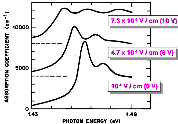
Fig. 9. Optical absorption spectra for a GaAs/AlGaAs quantum well sample at room temperature for various electric fields applied perpendicular to the quantum well layers. The spectra are shifted vertically for clarity [9].
